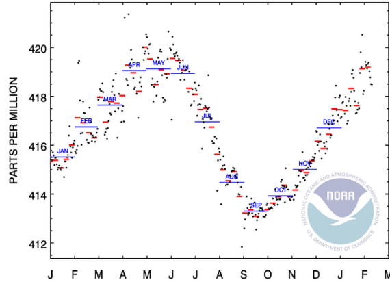
One year of CO 2 daily and weekly means at Mauna Loa
