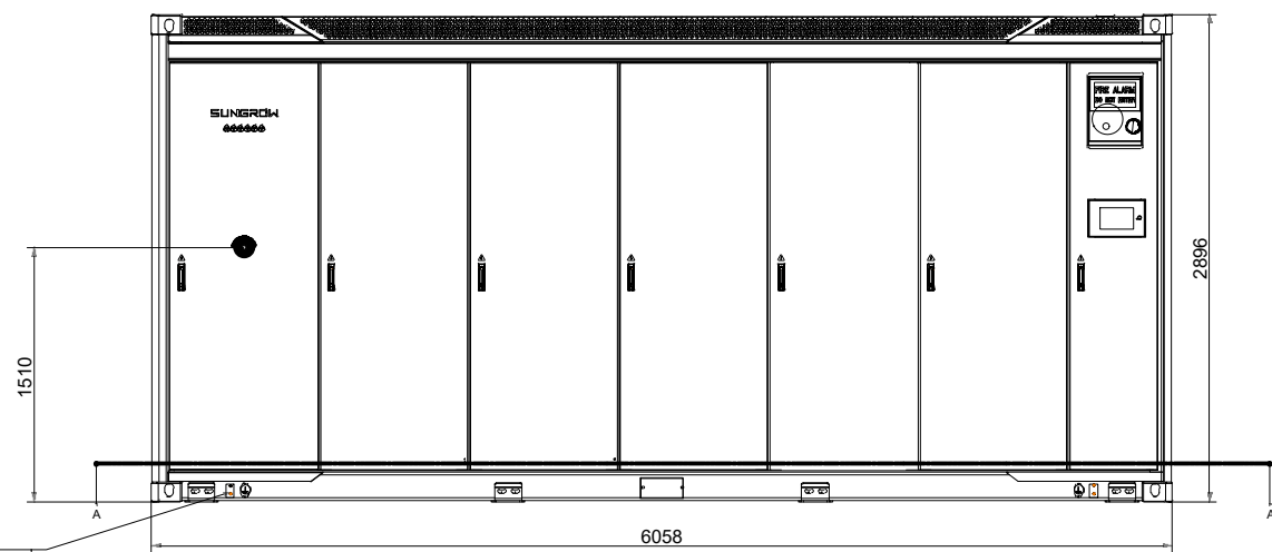
Vista frontal
